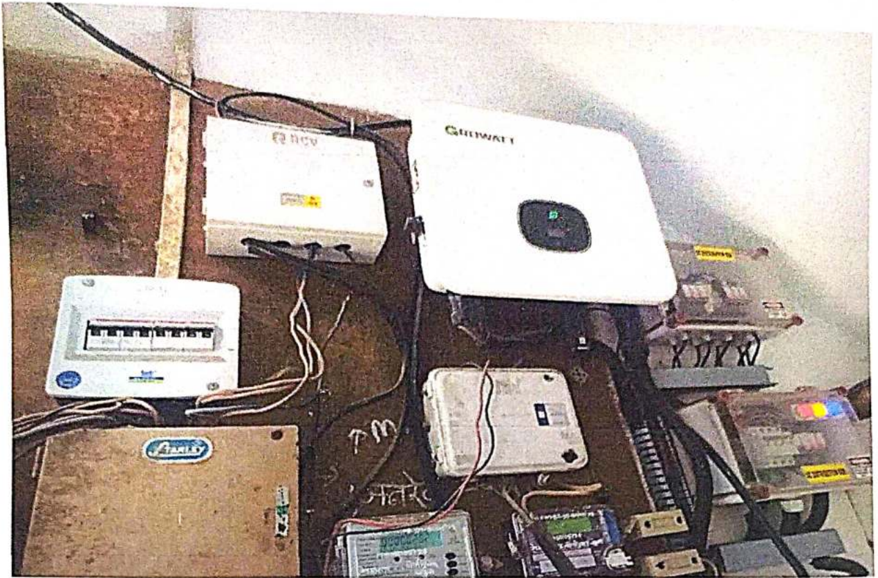
Electricity Supply By Using Solar Panels
